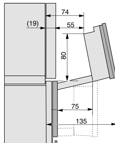
Detalle panel elevable
